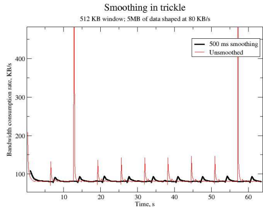
Figure 2: An illustration of the effect of smoothing in Trickle.
