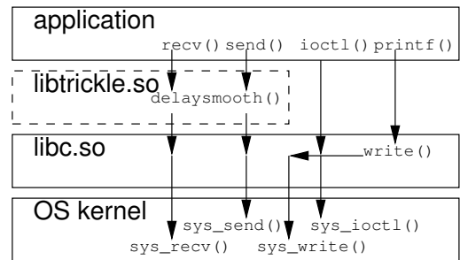
Figure 1: Illustrating the interpositioning mechanism.
